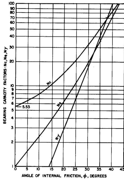
Figure 1 – Bearing Capacity Factors
